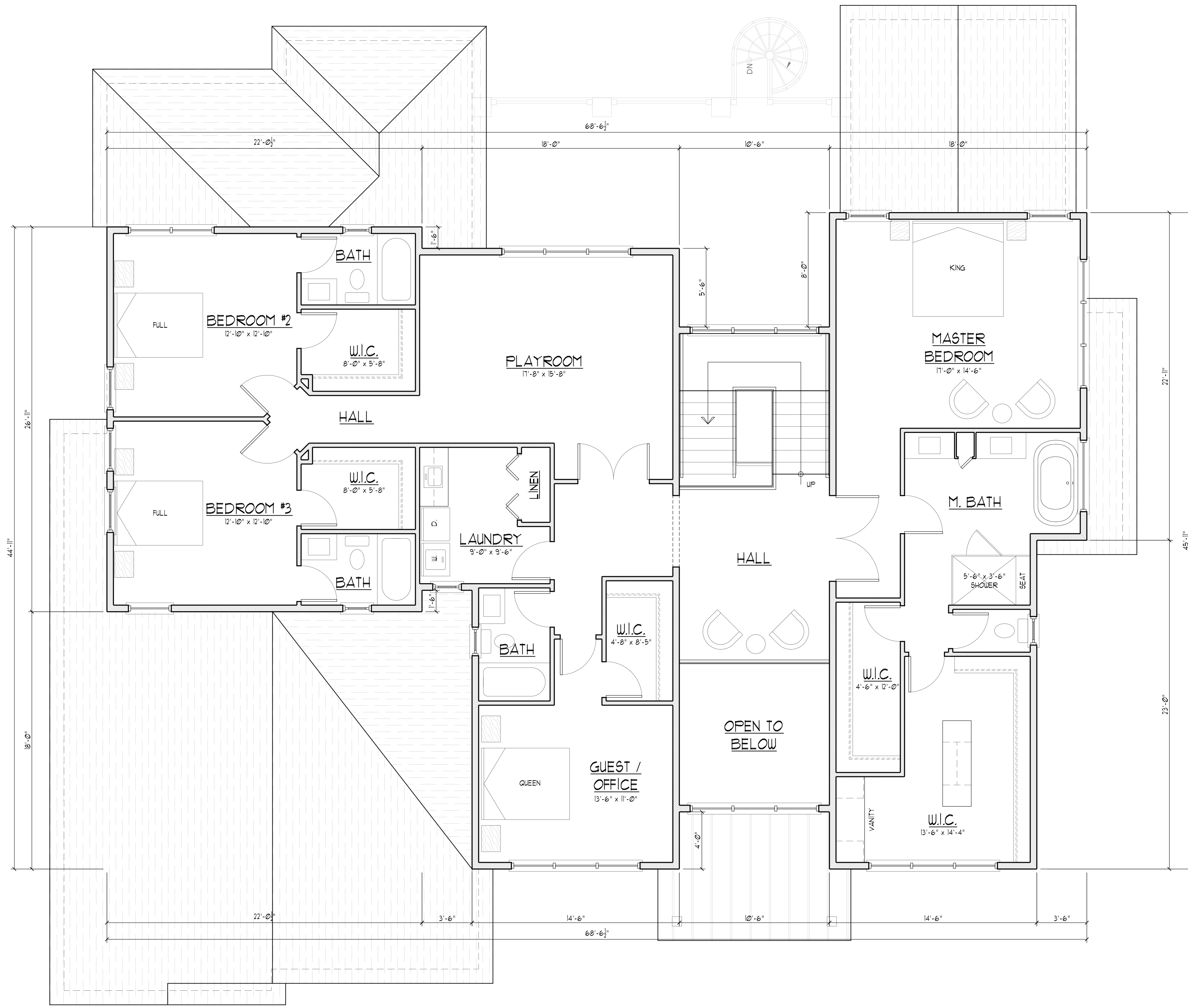
1 SECOND FLOOR PLAN A-3 1/4" x 1'-0"
