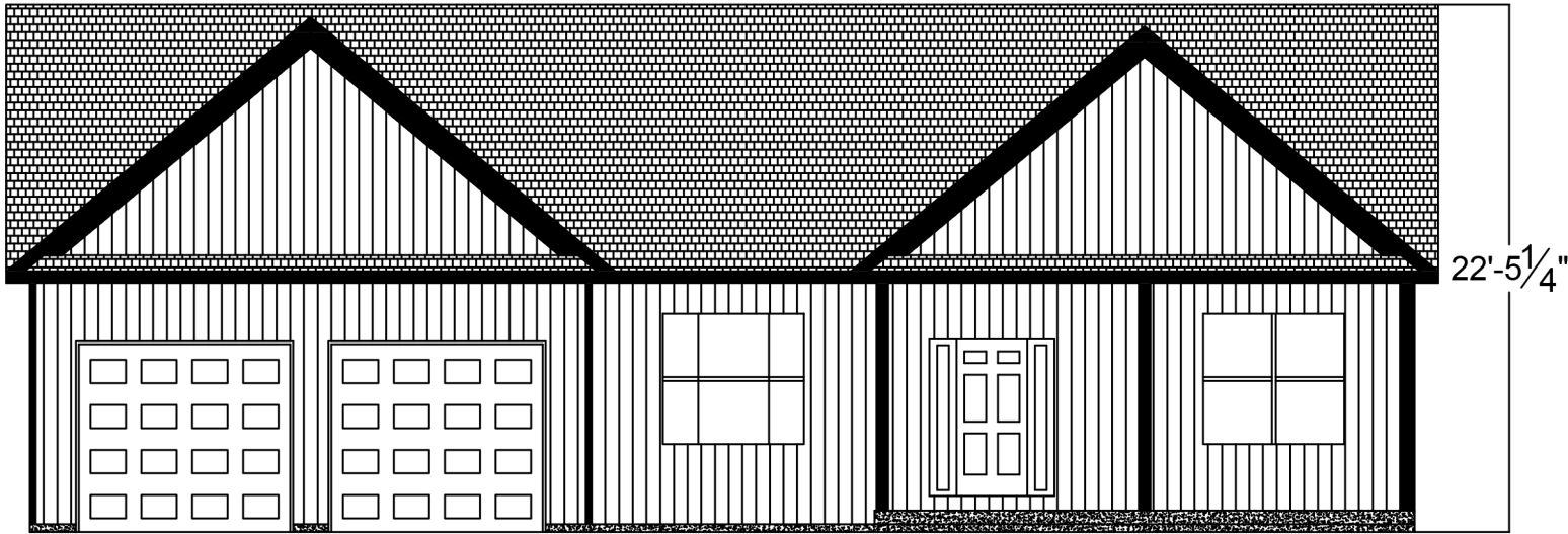
Elevation - Front
